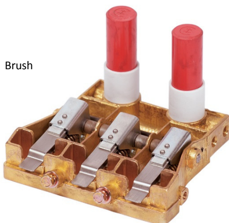
Brush Holder
